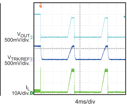
Over-Current
