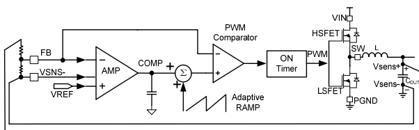
Figure 2: COT Control
